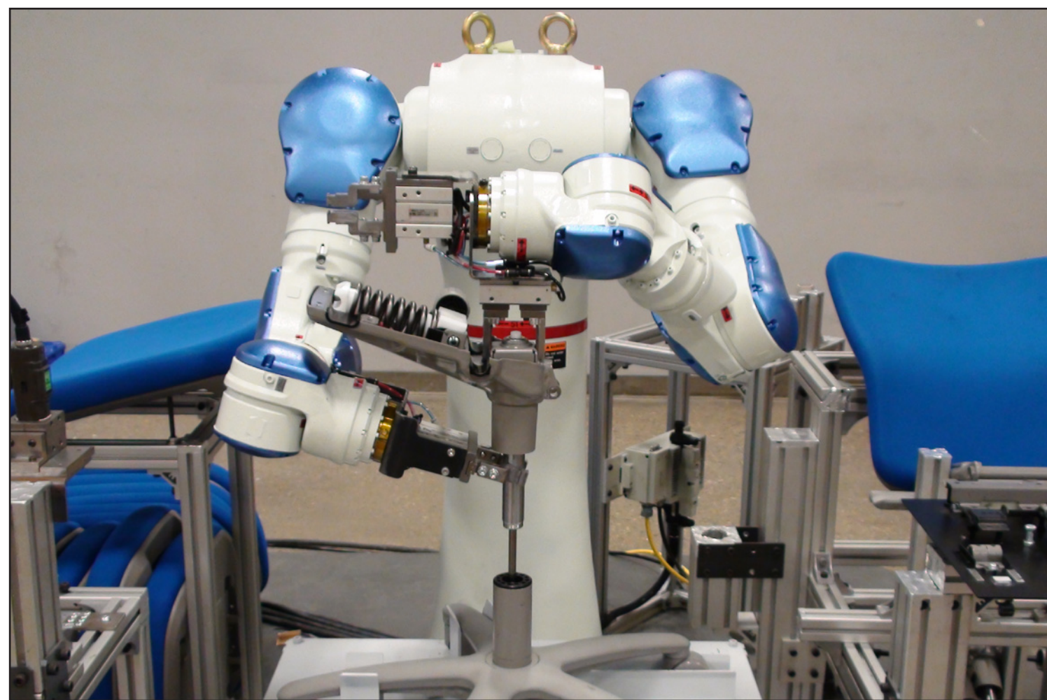
TWO ARMS POSITION SUBASSEMBLY INTO BASE
