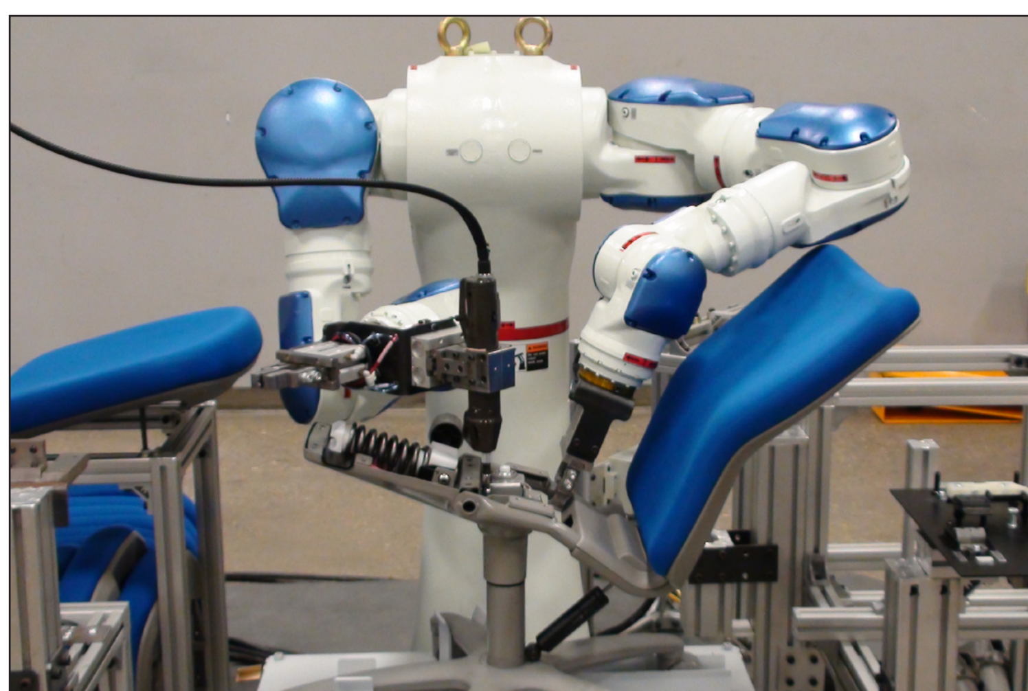
ONE ARM HOLDS CHAIR IN POSITION; SECOND ARM ATTACHES BRACKET
